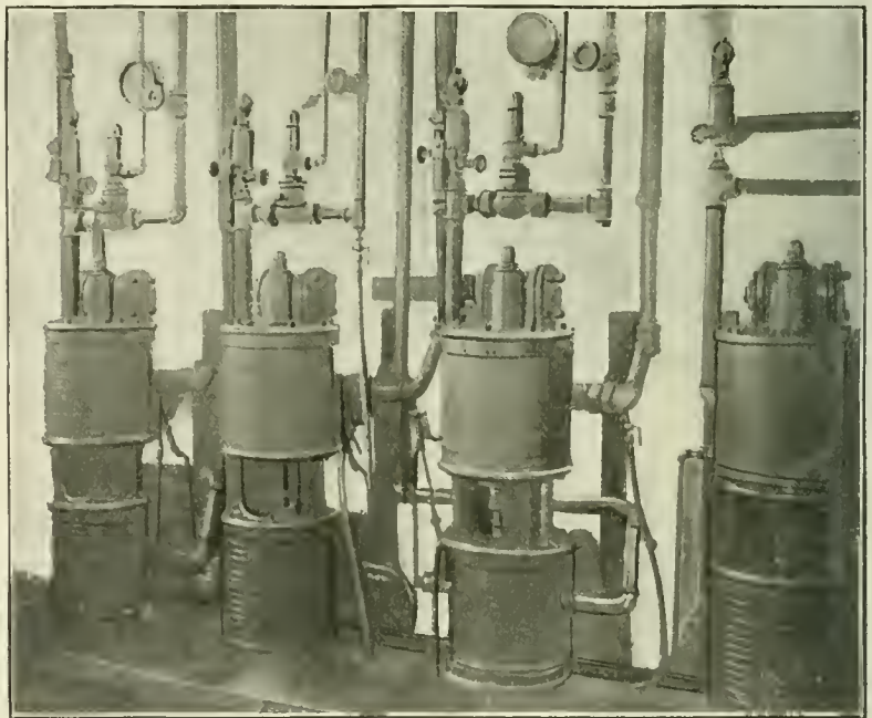
BATTERY OF AIR PUMPS IN PHILADELPHIA TESTING YARD OF THE READING RAILROAD.
